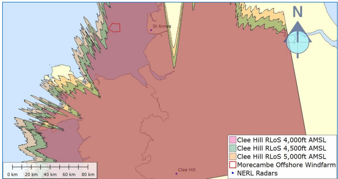
Figure 36: Cleve Hill PSR RLoS coverage at 4,000ft, 4,500ft and 5,000ft AMSL
